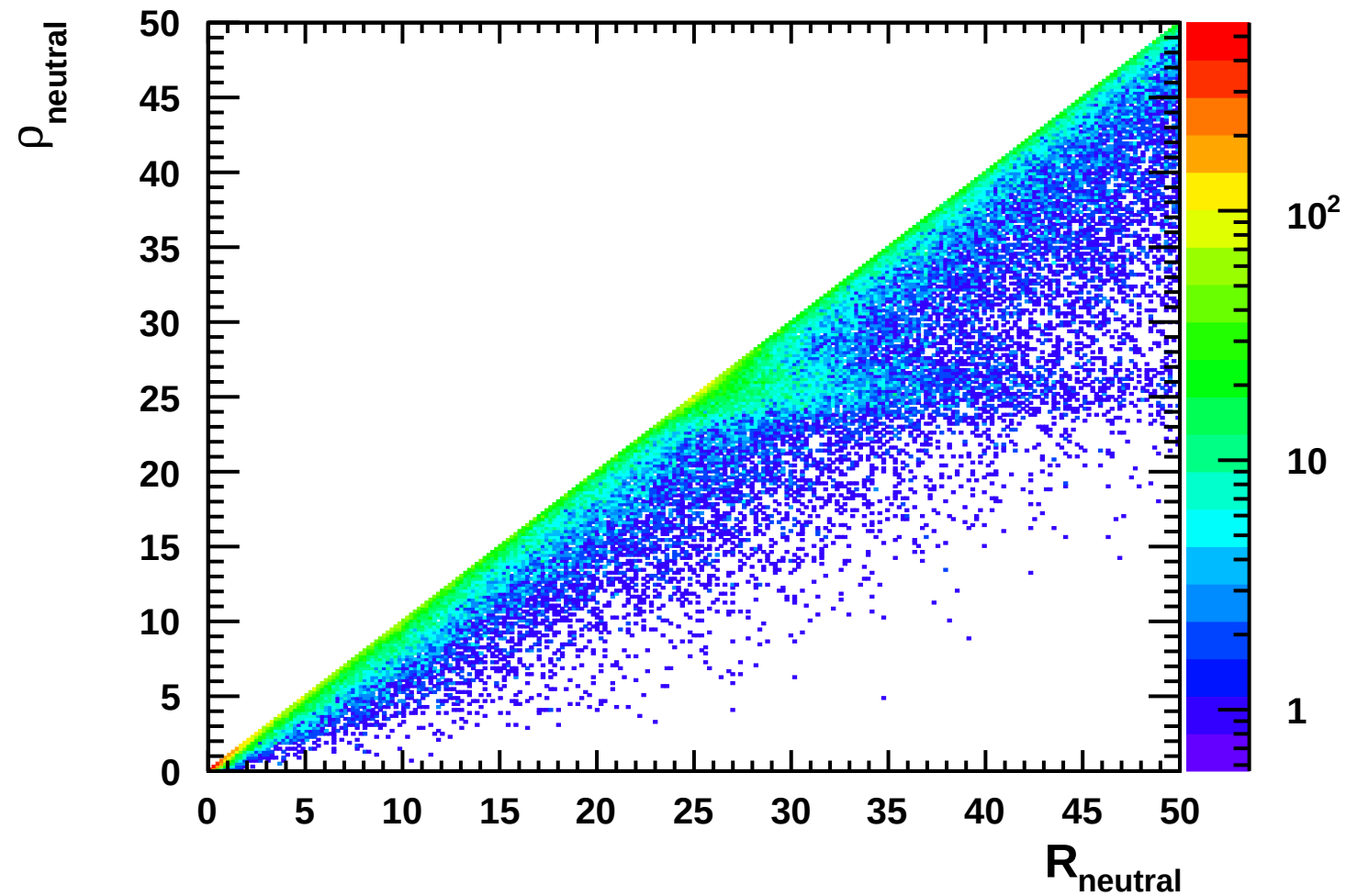
Rho Neutral vs R MC sum
